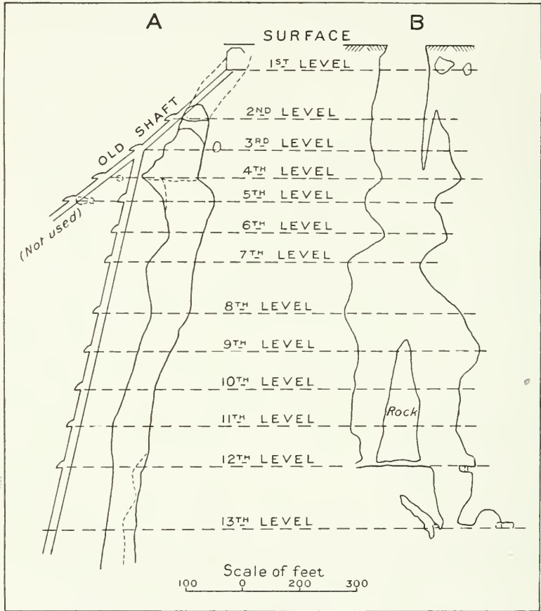
Fig. 57—Showing two sections through Copper Cliff mine, Copper Cliff, Ontario. A is a vertical section through shaft; B is a section at right angles to A. After A. P. Coleman.
